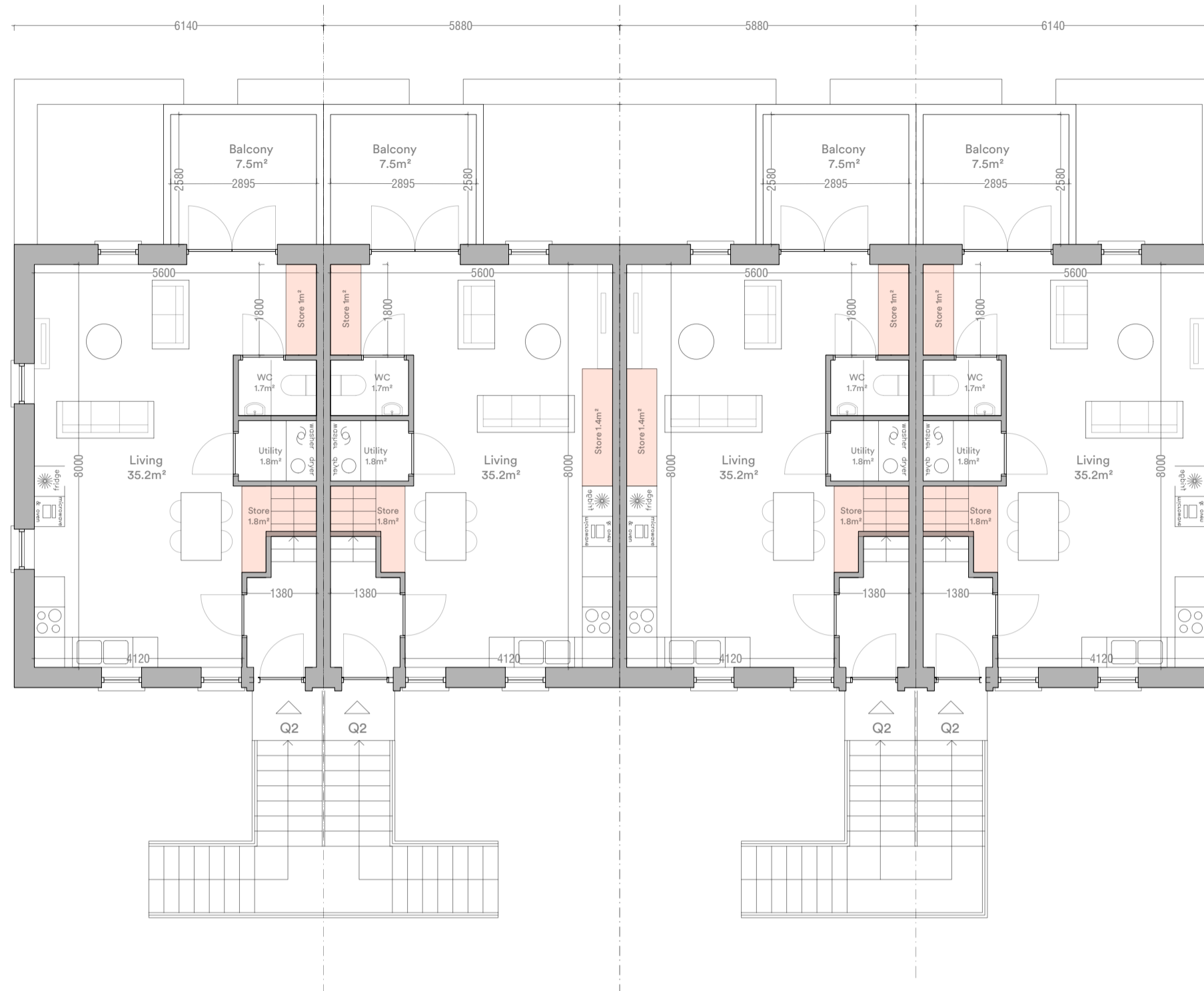
Duplex Block C First Floor
