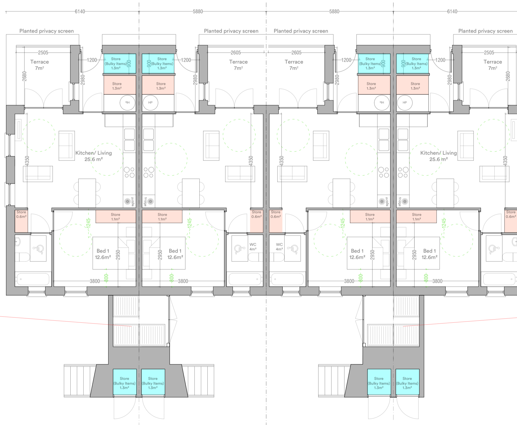
Duplex Block C Ground Floor
